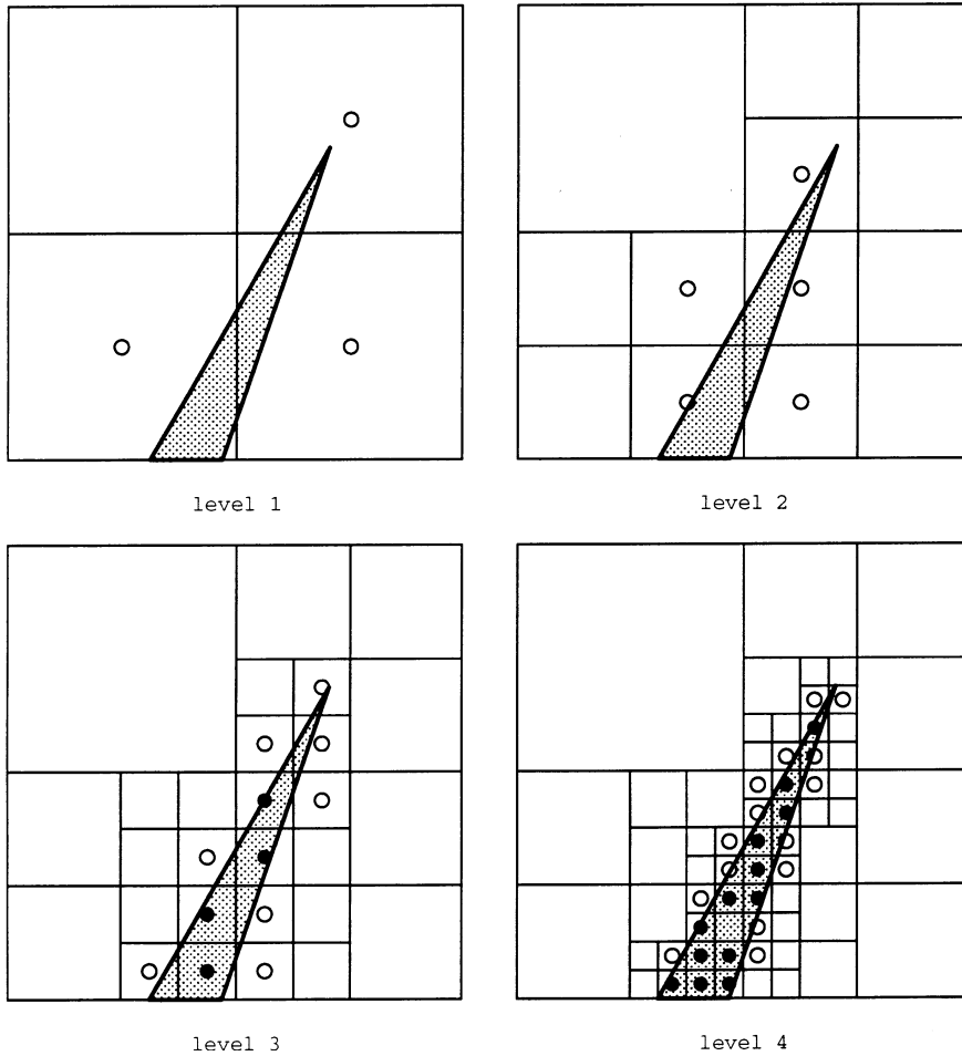
Figure 2: Intersection of thin object and pyray, showing adaptive subdivision at levels 1 to 4.
