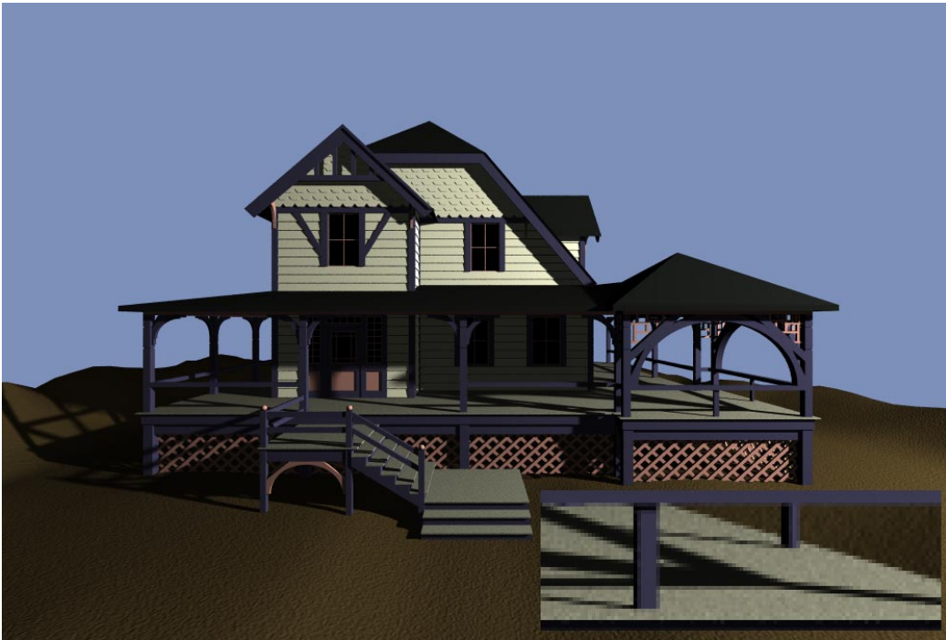
Figure 15: Same as last, but texture sampled 16 times per pixel. Quality: very good; time: 353.55 min. Time for similar image with stochastic sampling: 539.42 min. Shadow aliasing is improved.
