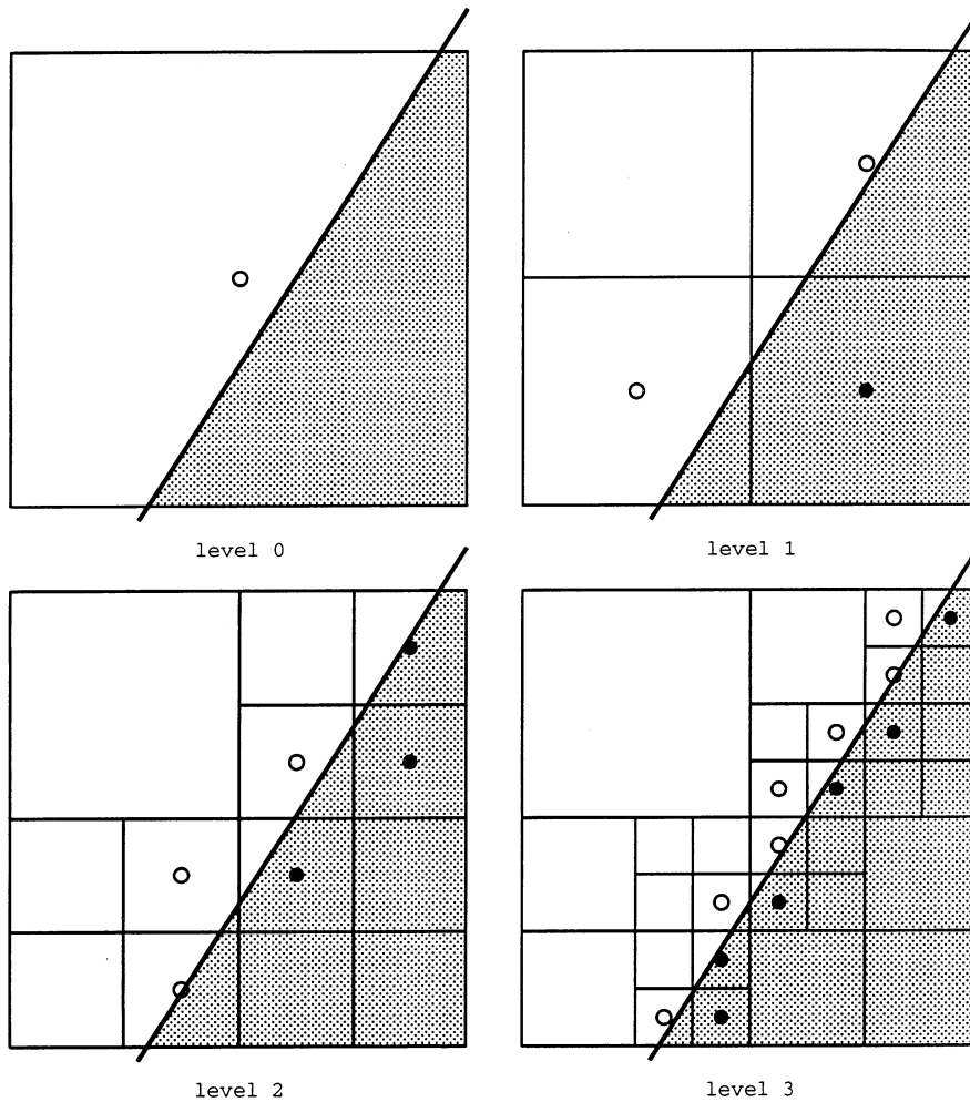
Figure 9: Intersection of object and pyray with one marginal edge, showing adaptive subdivision at levels 0 to 3.
