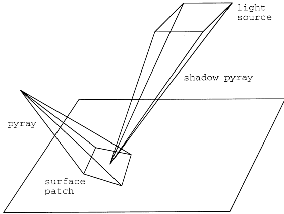
Figure 4: Shadow pyray from a surface point to a distributed light source.
