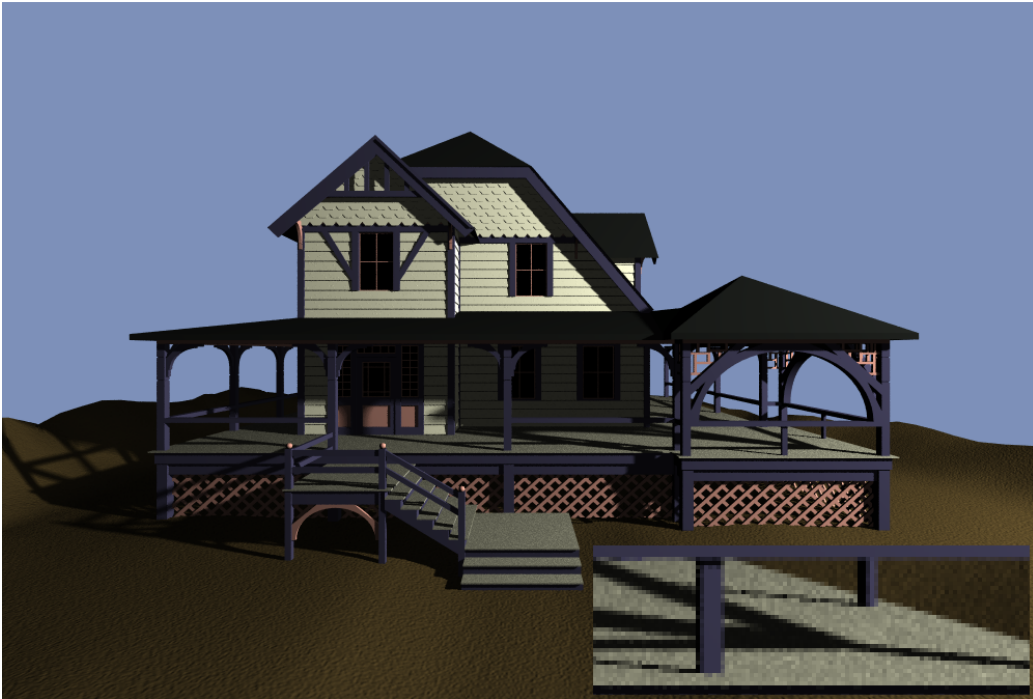
Figure 14: House with texture mapping rendered with ASOS ( MAX=2 , \epsilon=0 ) and texture sampled 4 times per pixel; quality: good; time: 158.01 min. Some shadow aliasing (enlarged) is noticeable.
