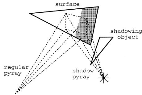
Figure 3: Generating accurate shadows from a point light source by casting a shadow pyray.
