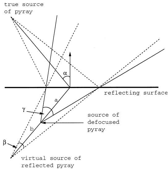
Figure 6: Defocusing a reflected pyray to produce blurred reflections.
