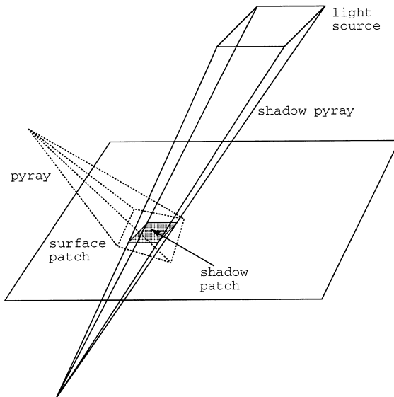
Figure 5: Extending the shadow pyray for improved sampling.
