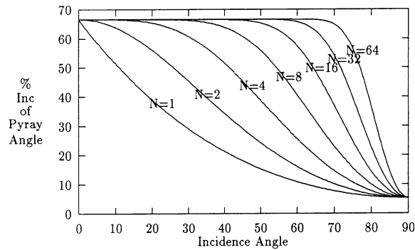
Figure 7: Percentage increase of angle of defocused pyray over original angle of pyray (taken as 2^\circ ), plotted as a function of the incidence angle, for various values of N , with DFR_{MIN}=0.6 and DFR_{MAX}=0.95 .
