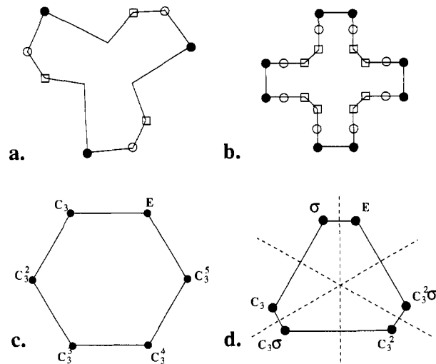
Figure 19. Divisions and orderings: (a) C_3 -symmetric configuration of cyclic connected points. Each set of differently marked points (●, ○, and □) is C_3 -symmetric. Each set is interlaced within the other sets. (b) D_4 -symmetric configuration of cyclic connected points. Each set of differently marked points (●, ○, and □) is D_4 -symmetric. Each set is inversely interlaced in the other sets. (c) C_6 -symmetric configuration of cyclic connected points and the associated symmetry element. (d) D_4 -symmetric configuration of cyclic connected points and the associated symmetry element.
