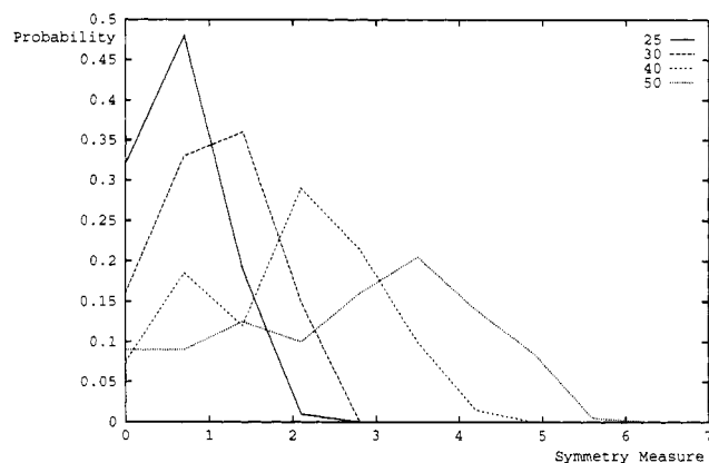
Figure 15. Probability distribution of the symmetry measure S(T_d) of a vibrating tetrahedron with random phase shifts associated with each arm. The distributions are given for several values of the maximum extension of the vibrations: 25, 30, 40, and 50% of original arm length. to a maximum of 25% of the original arm length and the other two arms to a maximum of 25% at a phase delay of 180^\circ . The CSM behavior indeed follows physical intuition: the symmetry measure reaches a maximum at the two extremes (two arms extended and two arms contracted to the maximum) and returns to a minimum at midcycle when the configuration is the original tetrahedral configuration. The overall shape of the curve of S follows the sinusoidal shape of the vibration.
